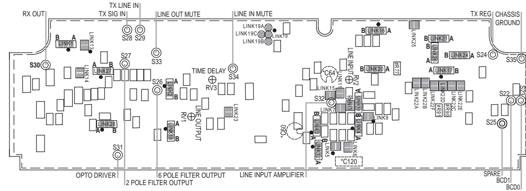
Figure 2: T2000-A80 PCB Links (PCB bottom side shown)
